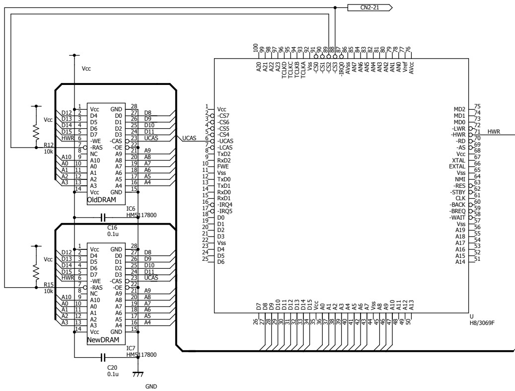
H8-3069net DRAM expansion Rev 1.0
